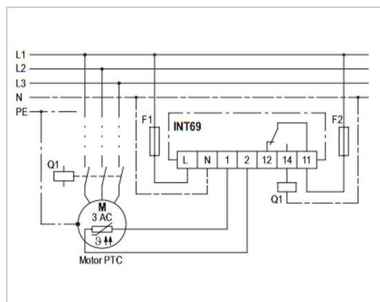
Wiring diagram
