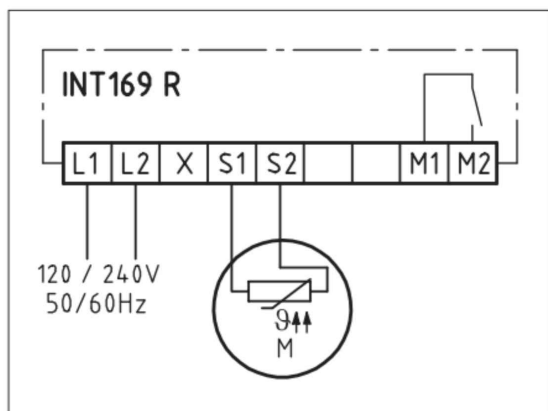
Connection diagram
