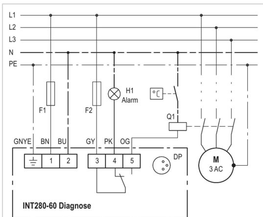
Wiring diagram
